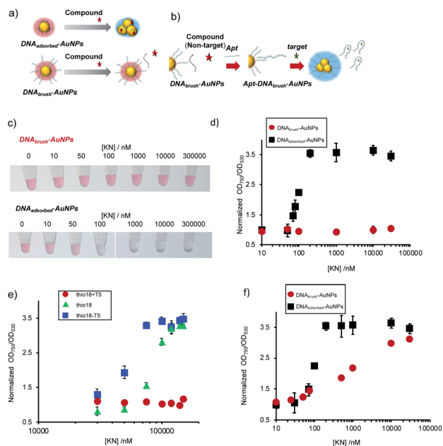
Fig. 1 Inhibition of non-specific AuNP aggregation by dense thiol DNA modification. (a) Schematic of the aggregation of AuNPs when DNA was immobilized on the surface by physical adsorption ( \text{DNA}_{\text{adsorbed}}\text{-AuNPs} ). AuNP surface modification with a DNA brush (Au–S bonds) ( \text{DNA}_{\text{brush}}\text{-AuNPs} ) to inhibit non-specific aggregation by compounds such as KN. (b) Schematic of the surface modification with an aptamer hybridized to the immobilized DNA brush for the detection of a target substance. (c) Typical photos of the AuNPs at increasing KN concentrations (between 0–30 000 nM) showing aggregation when the DNA was only immobilized by physical adsorption ( \text{DNA}_{\text{adsorbed}}\text{-AuNPs} ), whereas no aggregation was formed for \text{DNA}_{\text{brush}}\text{-AuNP} . (d) Normalized \text{OD}_{750}/\text{OD}_{530} values of the AuNP solutions. OD ratio without KN was defined as 1. The averaged values of three different samples tubes were shown. (e) Effect of KN on \text{DNA}_{\text{brush}}\text{-AuNP} with different lengths (thio18 – T5 (13 bases), thio18 (18 bases), thio18 + T5 (23 bases)). The same amount of DNA (approximately 1100 molecules) was immobilized on the AuNP surface. The averaged values of three different samples tubes were shown. (f) Effect of KN on \text{DNA}_{\text{brush}}\text{-AuNP} and \text{DNA}_{\text{adsorbed}}\text{-AuNP} with the same amount of DNA (approximately 100 molecules). The averaged values of three different samples tubes were shown.
